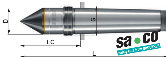
Form GV solid carbide point with safety core sa•co®
