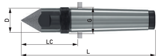
Form 255CA full centre 60°, with draw-off thread
